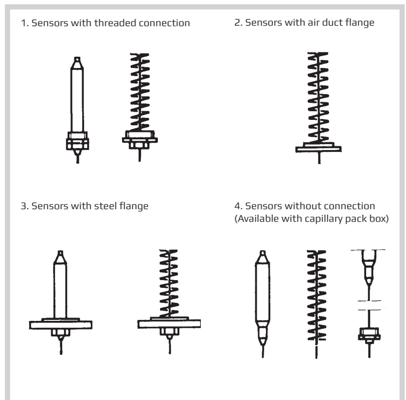
FIG. 4. SENSOR TYPES
