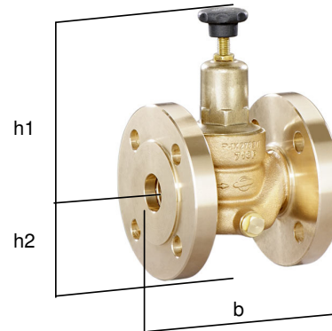
DN 15 - DN 32 (design DN 80 as below)
